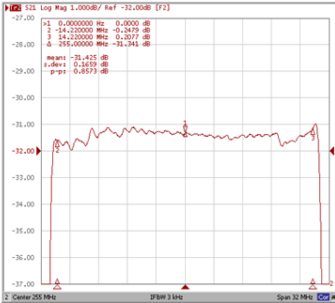
Ripple Variation Fo±14.22MHz
