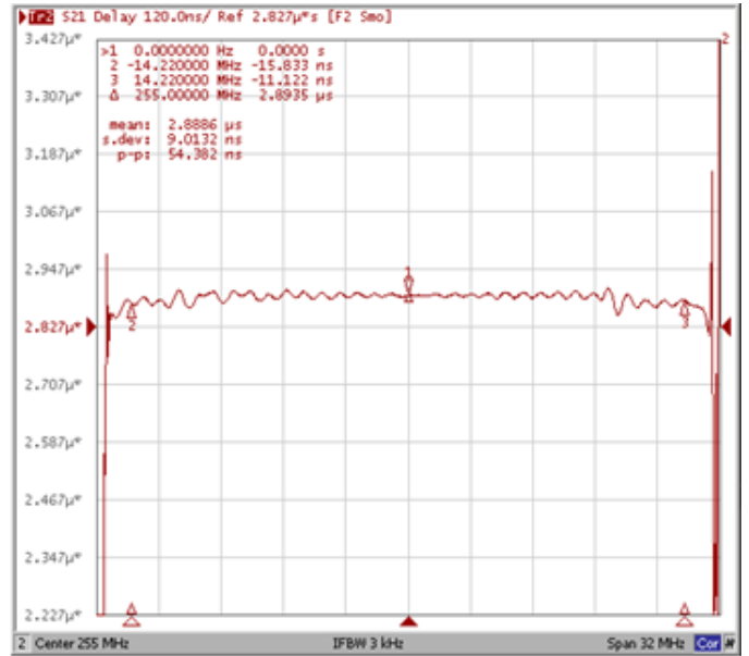
Group Delay Variation Fo±14.22MHz
